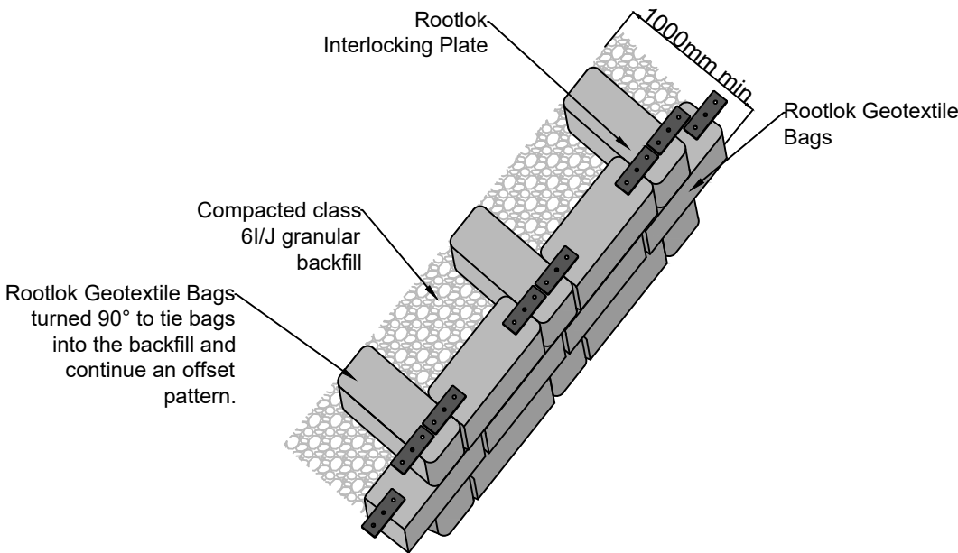
Typical Build
