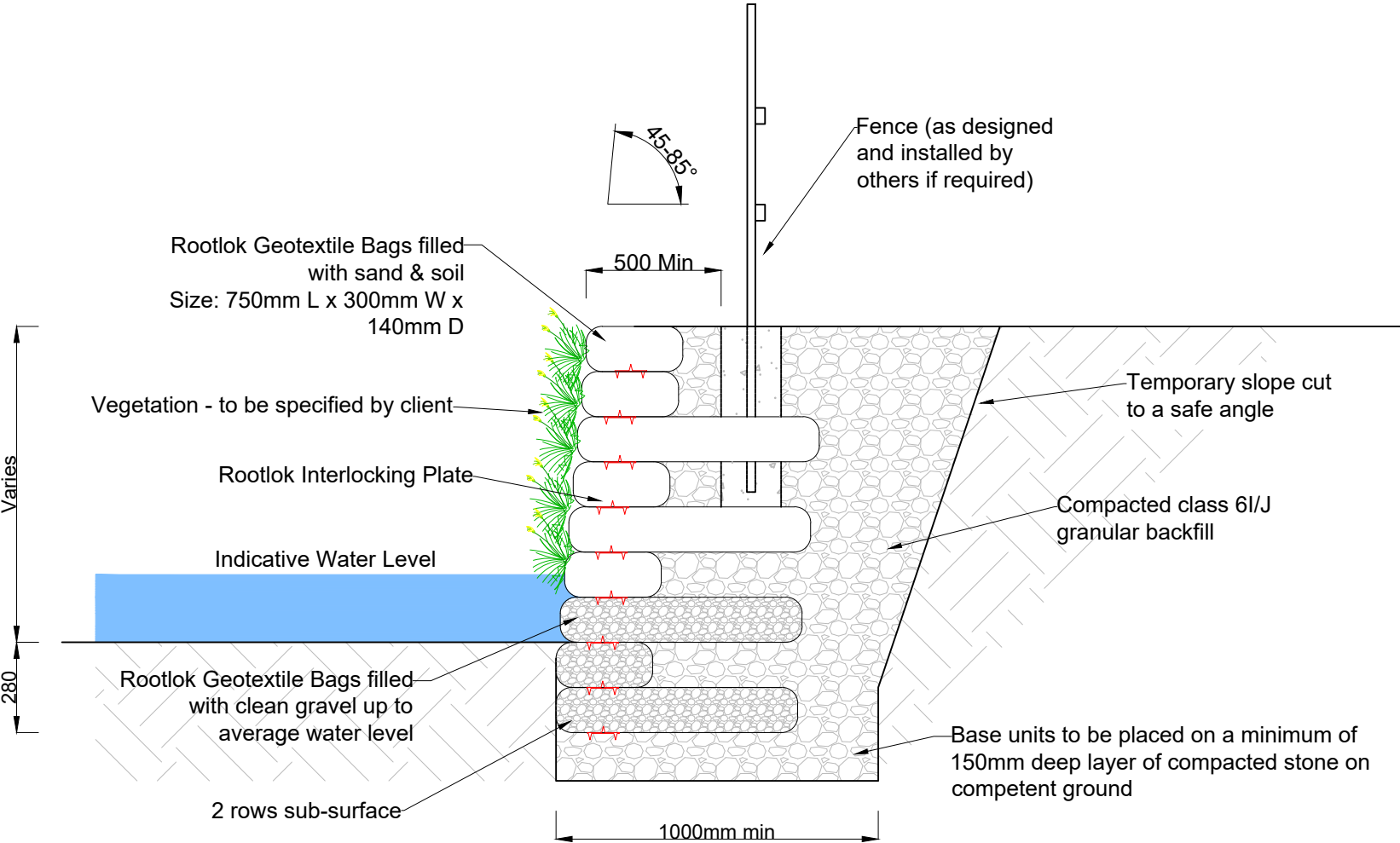
Typical Section
