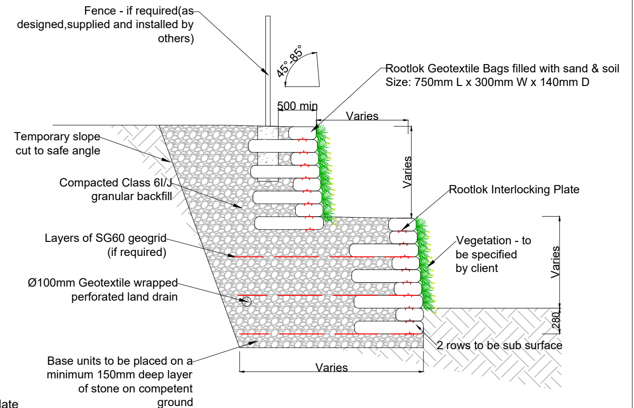
2 Tiered Wall Section View
