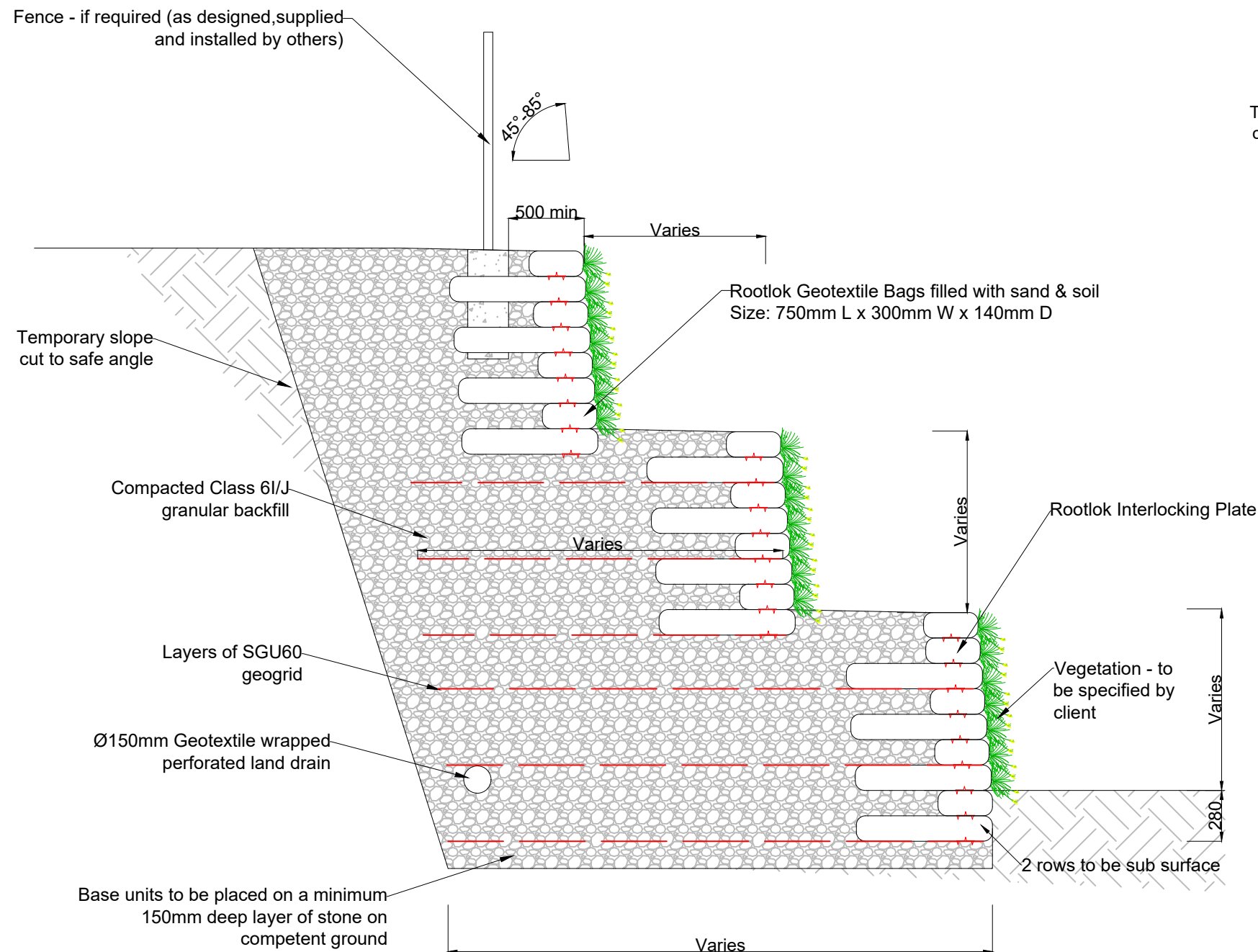
3 Tiered Wall Section View
