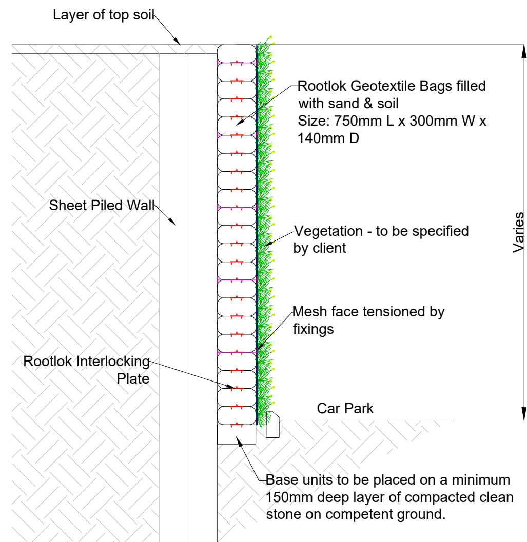
Typical Section
