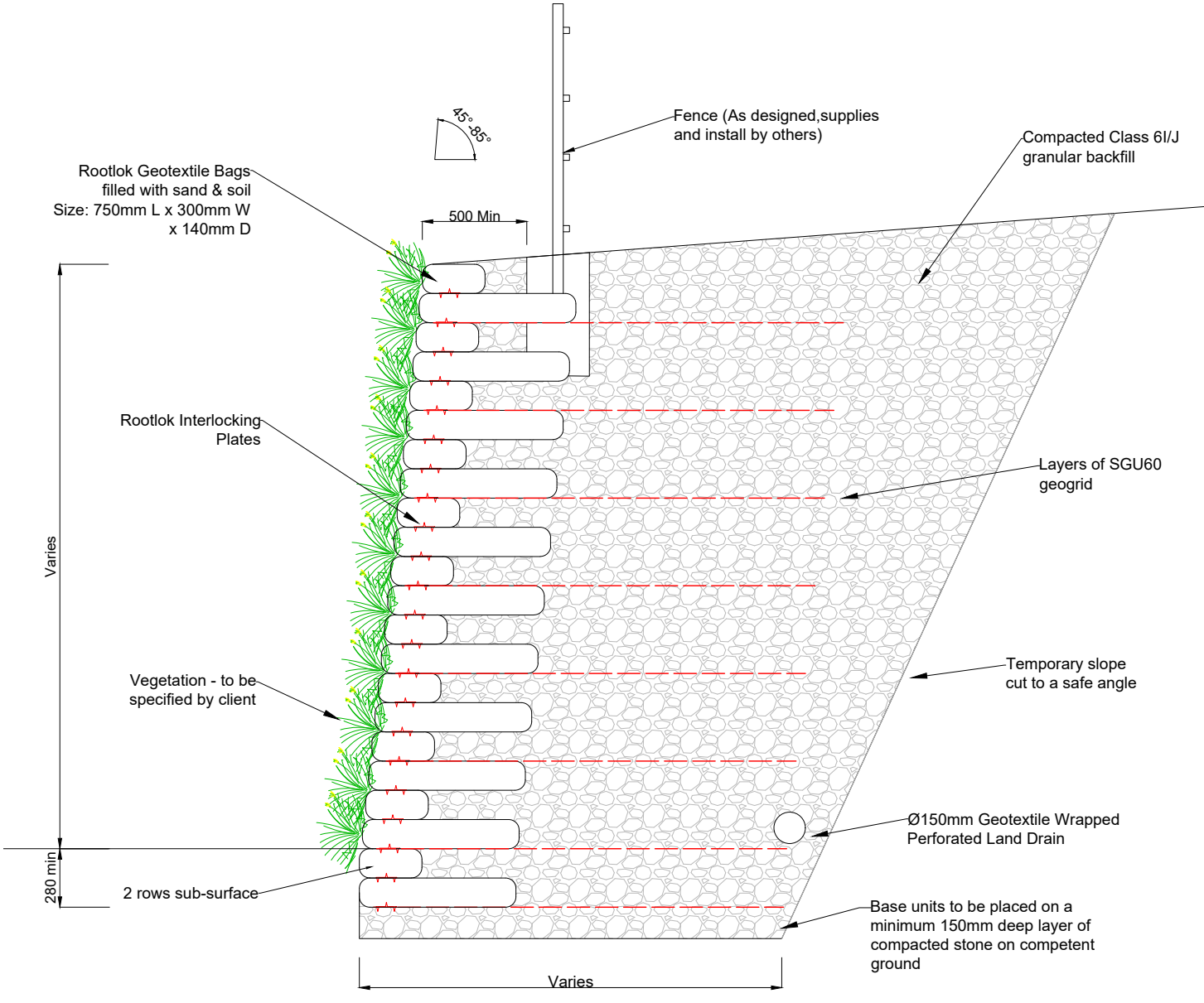
Typical Section - Tie Back with Geogrid
