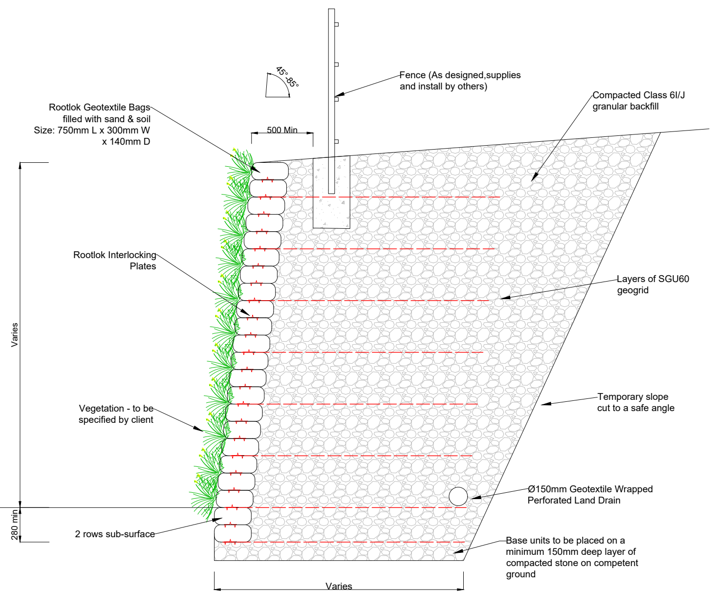
Typical Section - Gravity with Geogrid
