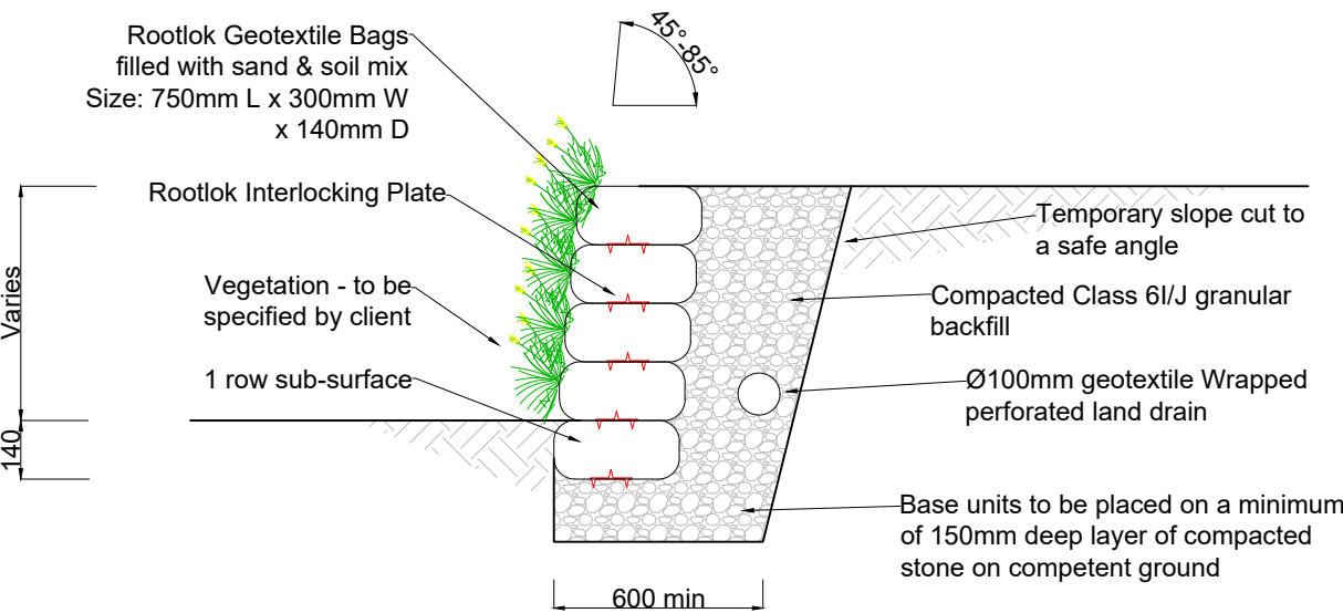
Gravity Wall 85° Batter
