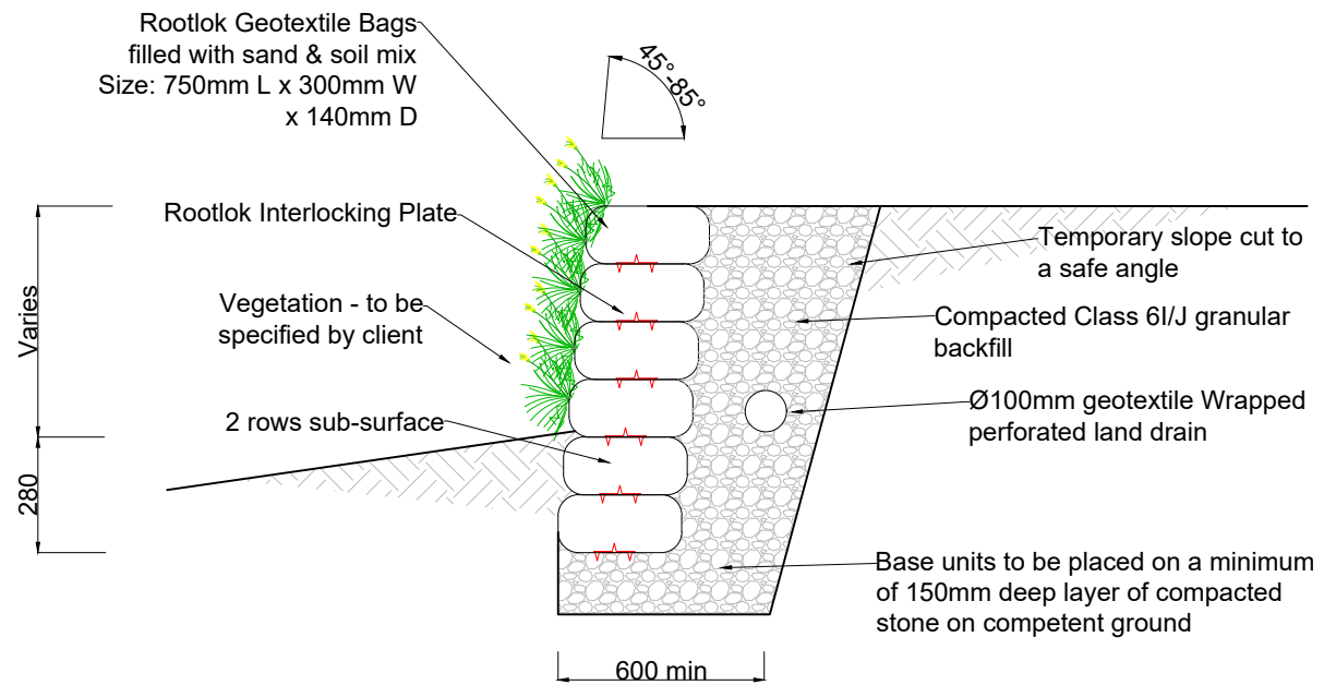
Gravity Wall 85° Batter (Toe Slope)
