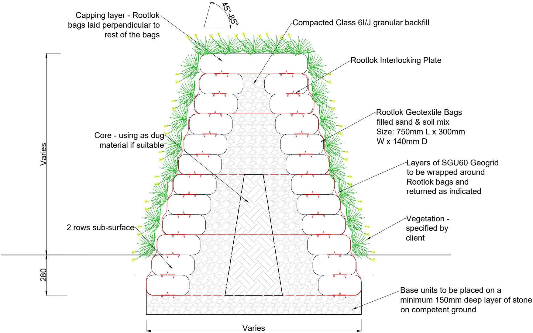
Typical Section
