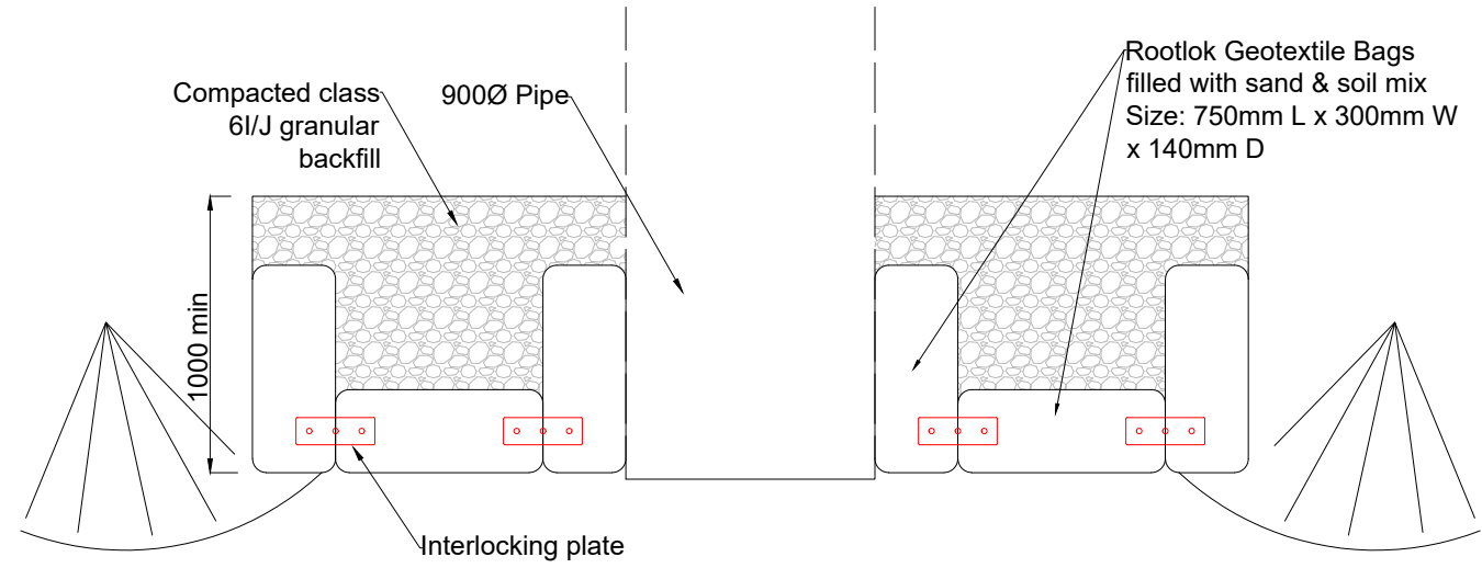
Plan View
