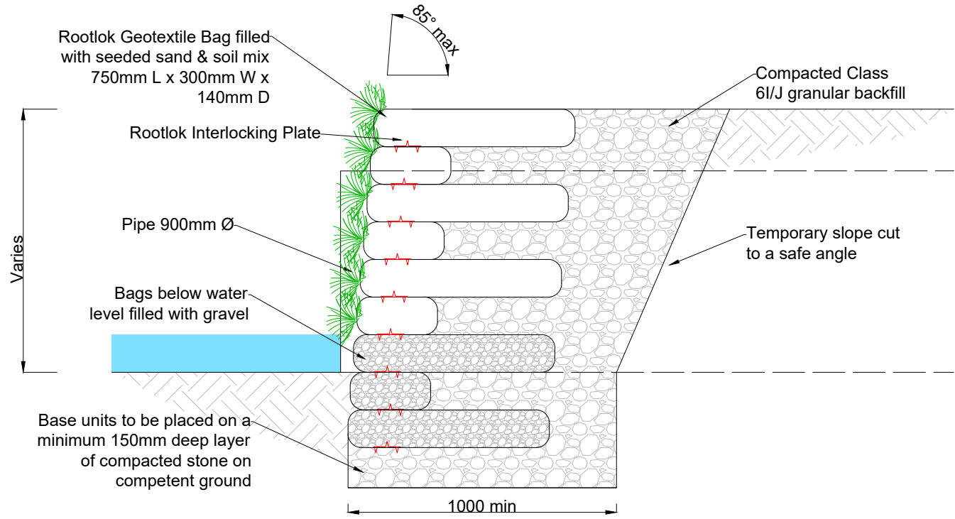
Section
