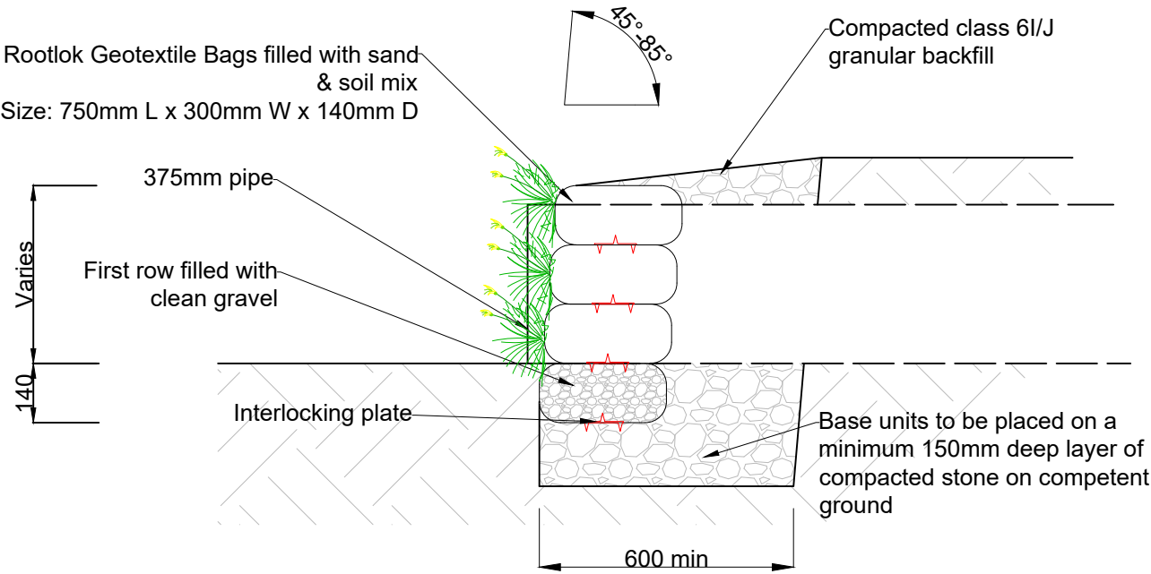
Typical Section
