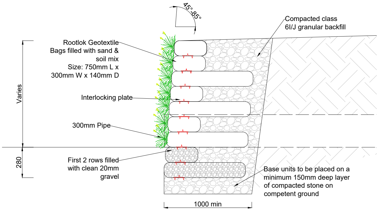
Section B-B
