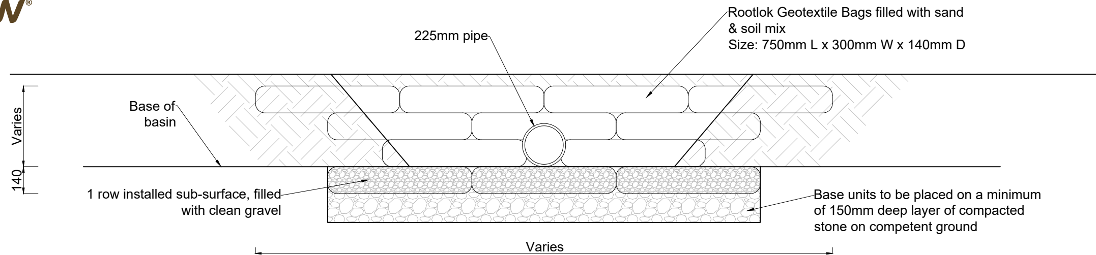
Typical Elevation
