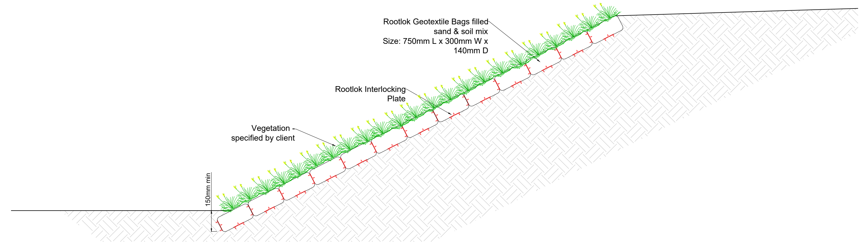
Typical Section
