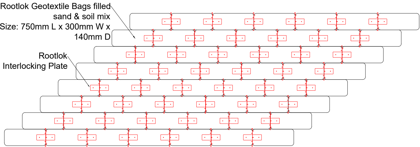
Typical Build
